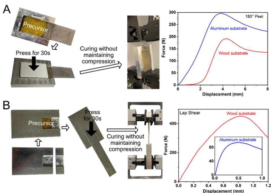
Fig. 5 (A) Peeling result of the cured ductile adhesive elastomer using a 180° peel setup. (B) Tensile result of the cured ductile adhesive elastomer using a lap shear setup.
