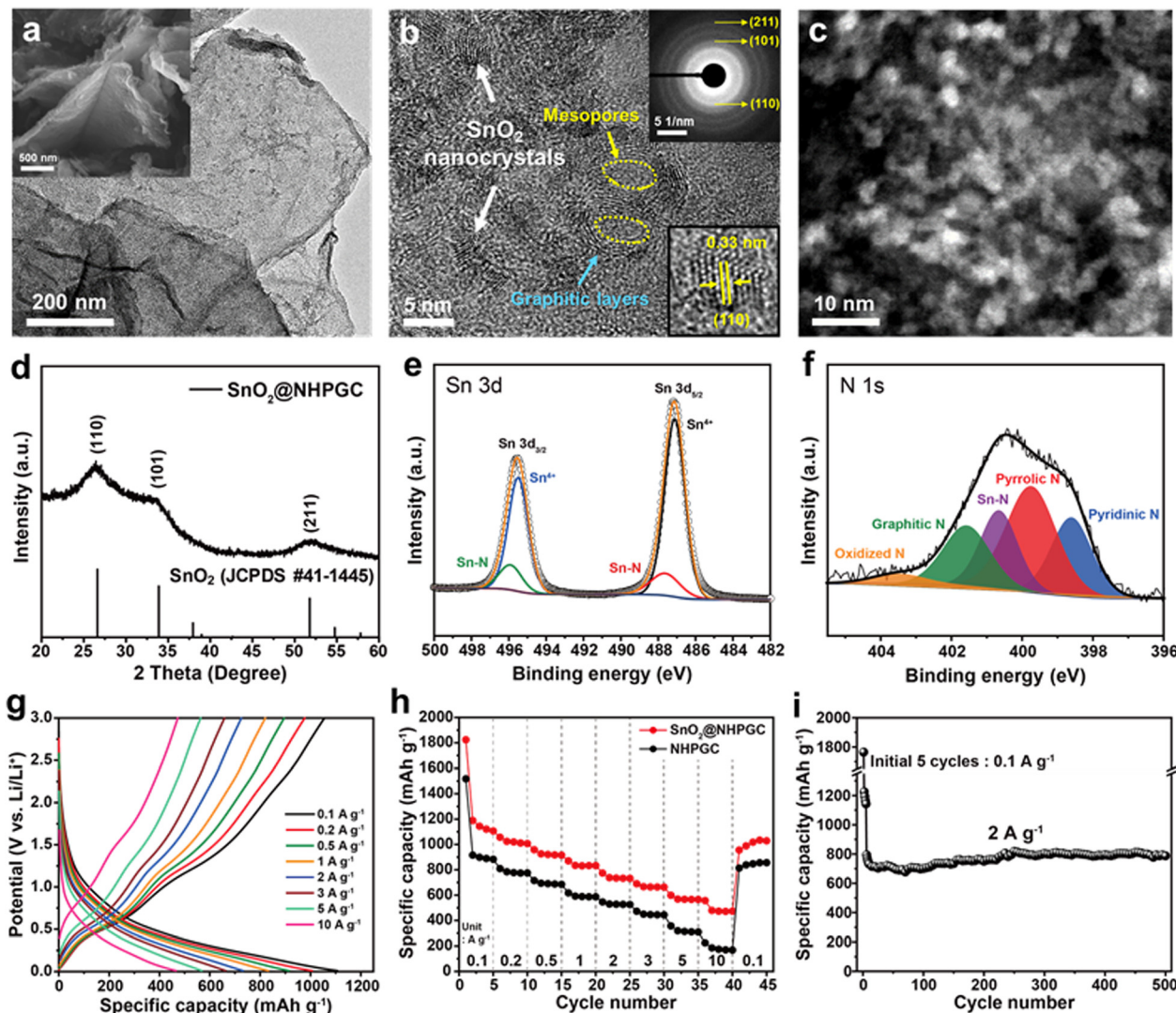
Fig. 4 The structural and electrochemical characterization of SnO 2 @NHPGC anode. (a) TEM and SEM (inset) images of SnO 2 @NHPGC. (b) HRTEM and (c) HAADF-STEM images of SnO 2 nanocrystals grown on NHPGC. Inset images in (b) show the SAED patterns for the HRTEM image (upper right) and lattice spacing of SnO 2 (lower right). (d) XRD patterns and (e) deconvoluted Sn 3d and (f) N 1s XPS spectra of SnO 2 @NHPGC. (g) GCD curves at different current densities, (h) rate performances compared to NHPGC, and (i) cycling performance of SnO 2 @NHPGC anode.
