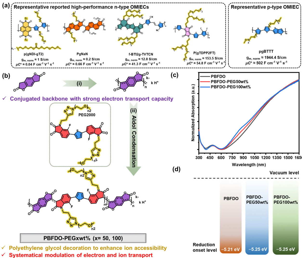
Fig. 1 (a) The molecular structures of representative p- and n-type OMIECs. (b) Schematic illustration of synthesis of PBFDO-PEG based OMIECs. (i) TMQ, DMSO, 85^\circ\text{C} , 6 h and (ii) injection of PEG units, 85^\circ\text{C} , 8 h. (c) Optical absorption spectra of the investigated OMIECs. (d) The energy level diagram of PBFDO-PEG based OMIECs.
