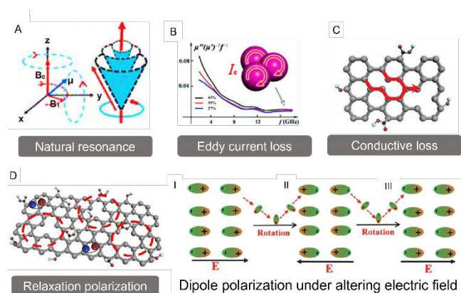
Fig. 1 The main magnetic and dielectric loss mechanisms of electromagnetic wave absorption. (A) Natural resonance. Reproduced with permission from ref. 10. Copyright (2020) Springer Nature. (B) Eddy current loss. Reproduced with permission from ref. 183. Copyright (2022) John Wiley and Sons. (C) Conductive loss and (D) polarization relaxation. Reproduced with permission from ref. 184. Copyright (2021) Elsevier. Of particularly note: the dipole polarization occurs in an alternating EM electrical field. Reproduced with permission from ref. 4. Copyright (2022) Elsevier.
