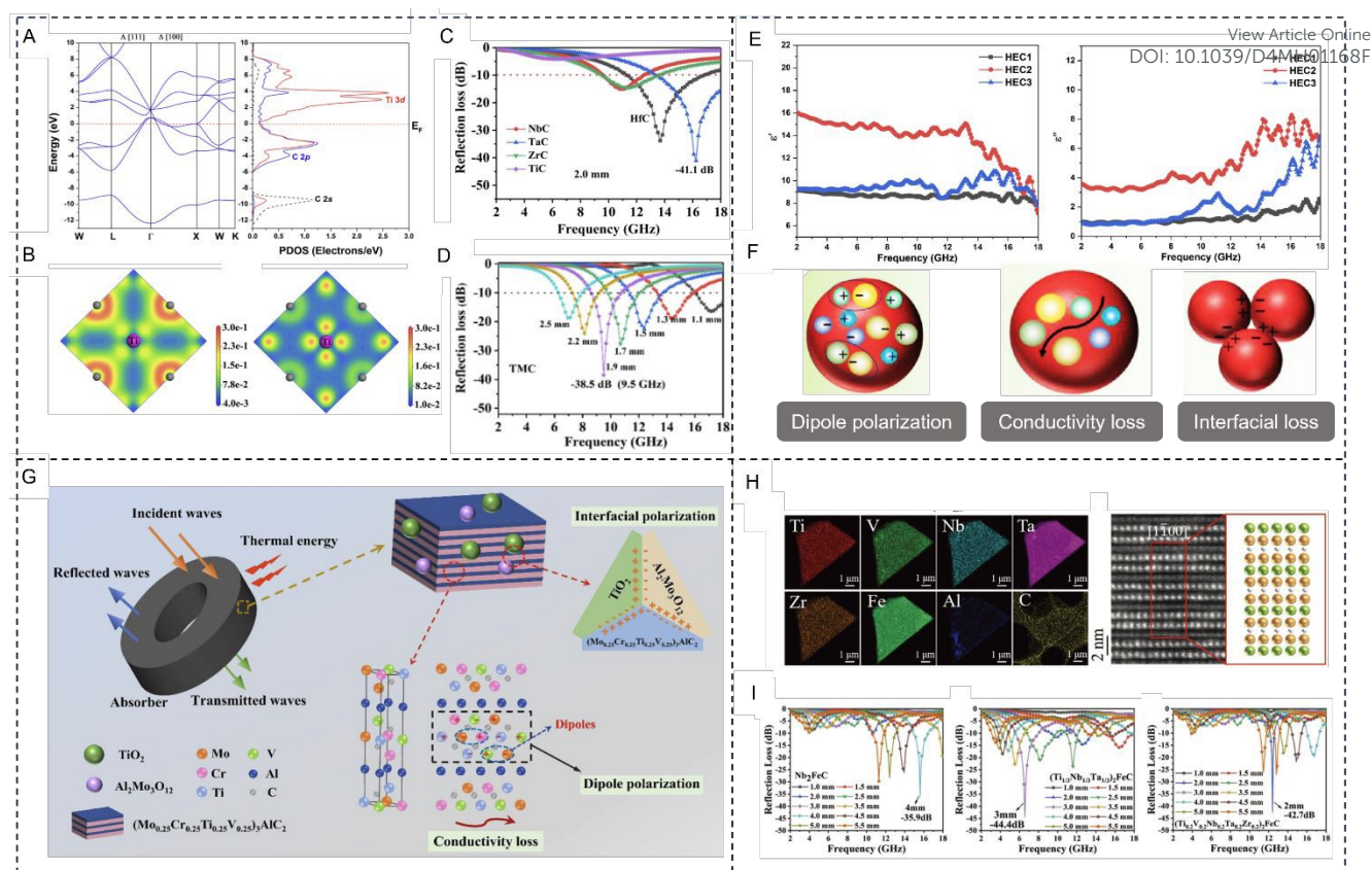
Fig. 7 High-entropy carbides for electromagnetic wave absorption applications. (A) Electronic structure (left) and partial density of states (right), (B) Low energy t_{2g} (left) and high energy e_g (right) levels of TiC, (C) comparison of reflection loss values of TMCs (TM=Ti, Zr, Hf, Nb, Ta), and (D) frequency dependence of reflection loss values of high-entropy (\text{Ti}_{0.2}\text{Zr}_{0.2}\text{Hf}_{0.2}\text{Nb}_{0.2}\text{Ta}_{0.2})\text{C} . Reproduced with permission from ref. 124. Copyright (2021) Elsevier. (E) Frequency-dependent real part and imaginary part of permittivity of (\text{Ti}_{0.2}\text{Zr}_{0.2}\text{Hf}_{0.2}\text{Nb}_{0.2}\text{Ta}_{0.2})\text{C} , (\text{Ti}_{0.2}\text{Zr}_{0.2}\text{Mo}_{0.2}\text{Nb}_{0.2}\text{Ta}_{0.2})\text{C} and (\text{Ti}_{0.2}\text{Zr}_{0.2}\text{Cr}_{0.2}\text{Nb}_{0.2}\text{Ta}_{0.2})\text{C} high-entropy carbides (HEC1, HEC2 and HEC3), and (F) schematic illustration of the electromagnetic wave absorption mechanisms. Reproduced with permission from ref. 125. Copyright (2023) Elsevier. (G) Schematic illustration of the electromagnetic wave absorption behaviours and mechanisms for (\text{Mo}_{0.25}\text{Cr}_{0.25}\text{Ti}_{0.25}\text{V}_{0.25})_3\text{AlC}_2 high-entropy MAX phase. Reproduced with permission from ref. 126. Copyright (2023) Elsevier. (H) Aberration corrected scanning transmission electron microscopy imaging and atomic lattice-resolved energy dispersive X-ray spectroscopy analysing of (\text{Ti}_{0.2}\text{V}_{0.2}\text{Nb}_{0.2}\text{Ta}_{0.2}\text{Zr}_{0.2})_2\text{FeC} in [1\bar{1}00] direction. The yellow, green, and gray balls represent atoms in the M-, A-, and X-sites, respectively. (I) Reflection loss curves of \text{Nb}_2\text{FeC} , (\text{Ti}_{1/3}\text{Nb}_{1/3}\text{Ta}_{1/3})_2\text{FeC} , and (\text{Ti}_{0.2}\text{V}_{0.2}\text{Nb}_{0.2}\text{Ta}_{0.2}\text{Zr}_{0.2})_2\text{FeC} . Reproduced with permission from ref. 127. Copyright (2021) Springer Nature.
