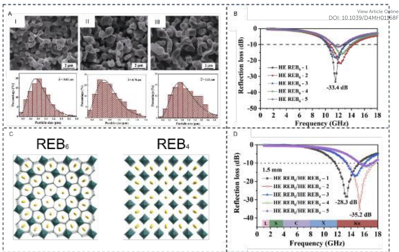
Fig. 8 High-entropy borides for electromagnetic wave absorption applications. (A) Scanning electron microscopy images and particle distributions of I: TMB 2 -1 (TM = Zr, Hf, Nb, Ta), II: high-entropy TMB 2 -2 (TM = Ti, Zr, Hf, Nb, Ta), and III: high-entropy TMB 2 -3 (TM = Cr, Zr, Hf, Nb, Ta), powders synthesized at 1950 °C for the dwelling time of 1 h. Reproduced with permission from ref. 128. Copyright (2023) John Wiley and Sons. (B) Comparison of reflection loss for HE REB 6 . Reproduced with permission from ref. 129. Copyright (2020) Springer Nature. (C) Crystal structure of REB 6 : RE atoms (yellow) and B 6 octahedron (teal) are arranged in a CsCl-like packing. REB 4 : Altering sheets of RE atoms (yellow) and B 6 octahedra (teal) linked by B 2 units forming a quasi-layer structure. (D) Comparison of reflection loss of high-entropy REB 6 /high-entropy REB 4 . Reproduced with permission from ref. 130. Copyright (2021) Elsevier.
