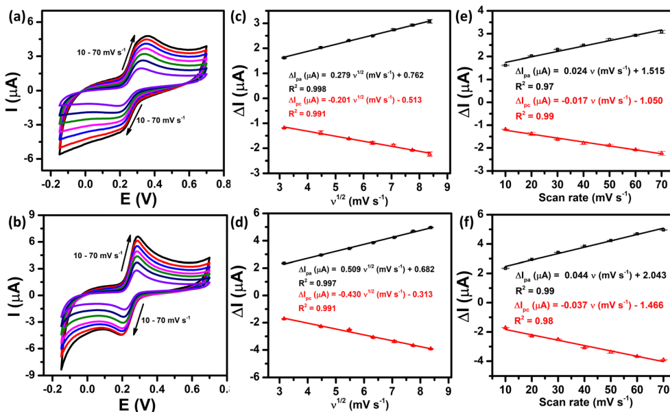
Fig. 5 CV curves recorded at the bare SPE and \text{ZnFe}_2\text{O}_4/\text{SPE} in 0.1 M PBS (pH 5.0) containing 50 \mu\text{M} PCM at different scan rates (a) and (b), plots of peak current vs. square root of scan rate (c) and (d), and plots of peak current vs. scan rate (e) and (f), respectively.
