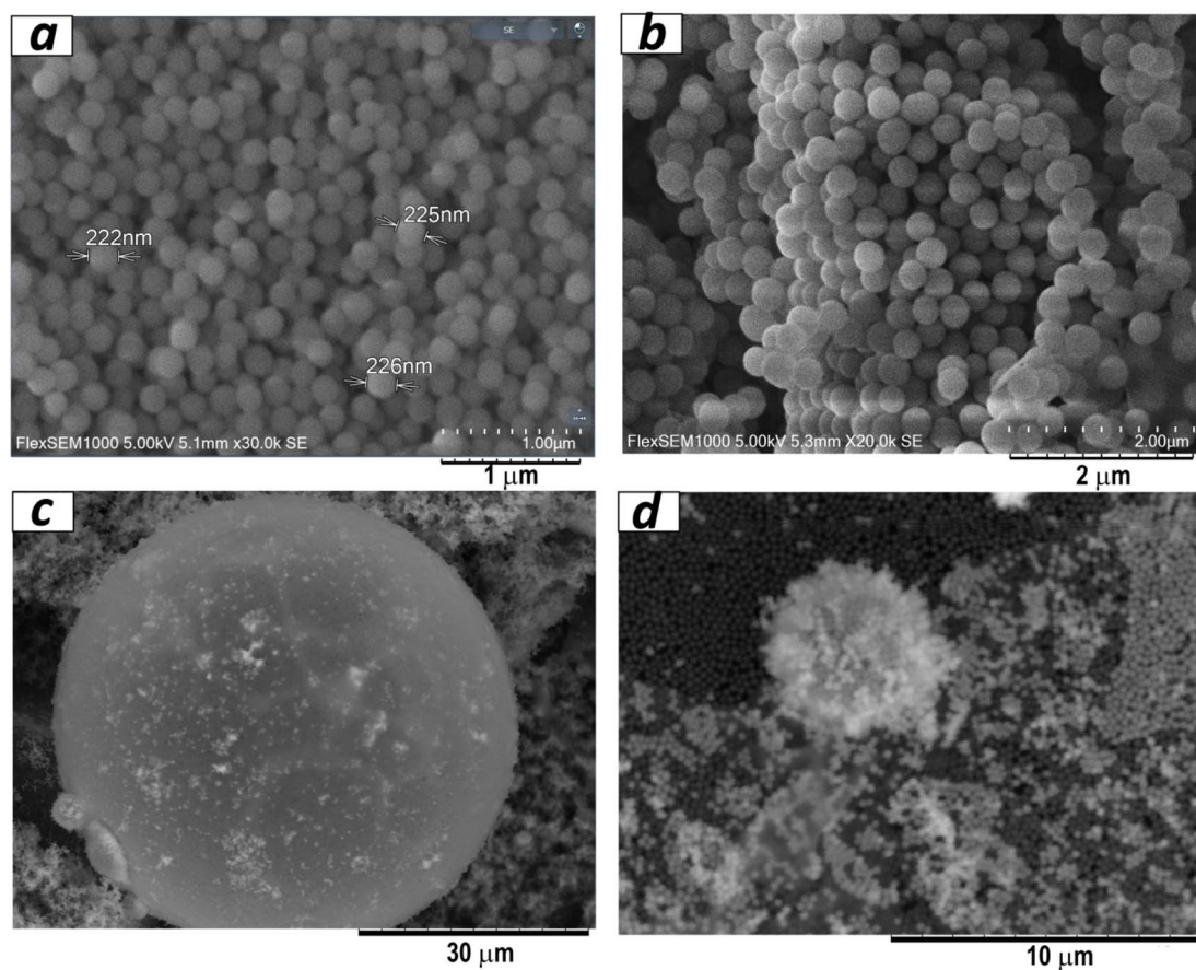
Fig. 2 SEM images of initial SiO 2 particles (a and b) and SiO 2 /–SH/–NH 2 particles (c and d).
