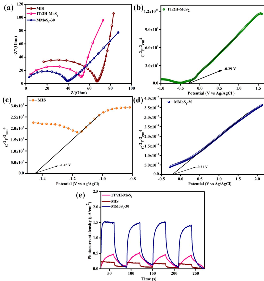
Fig. 4 (a) EIS plot of neat components and the prepared \text{MMoS}_2\text{-30} composite. Mott–Schottky plots of (b) 1\text{T}/2\text{H-MoS}_2 , (c) MIS and (d) \text{MMoS}_2\text{-30} . (e) Transient photocurrent measurement of neat 1\text{T}/2\text{H-MoS}_2 , MIS, and \text{MMoS}_2\text{-30} .
