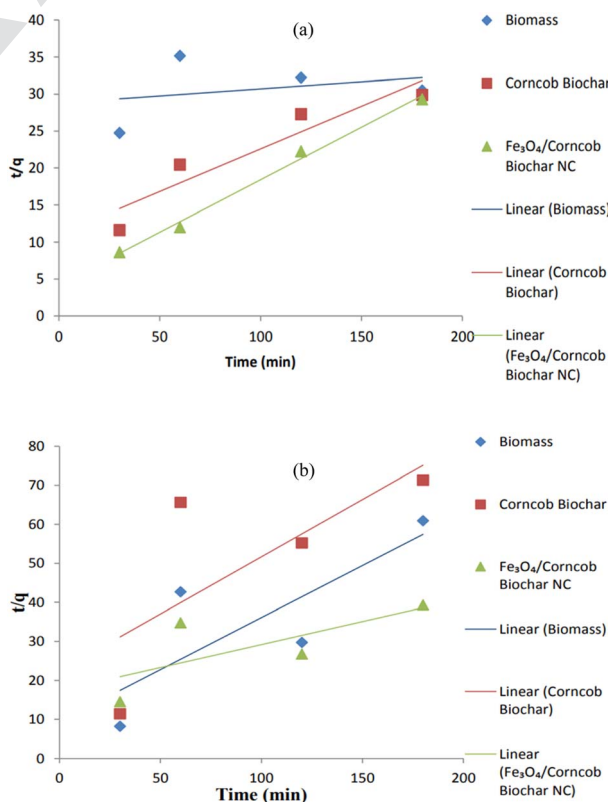
Fig. 16 Second order plot (a) Cr(IV) and (b) Ni(II).
