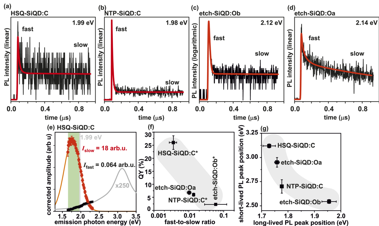
Fig. 4 (a–d) Examples of PL decays in a 1 \mu s window for the individual studied samples. Sample labels are noted at each panel. The black curves represent the measured data, the red curves are the fits. Please note the logarithmic vertical scale in panel (c), in which the logarithmic scale was necessary to visualize both components. To ensure that the results are comparable from one sample to another, all measurements were carried out using UV excitation (315–343 nm). (e) Spectral profiles of the long- and short-lived components deduced from the measurements shown in panel a, the spectral position of which is highlighted by the gray vertical line. The black and red datapoints show the \lambda dependence of the PL intensity of each of the components, the gray and orange curves are extrapolations used to estimate the overall PL intensity emitted in each of the bands. The shape of the spectra and the spectral position of each peak is known from other measurements, therefore, only the amplitude and possibly the width of the peak need to be fitted. In this sample, the PL peaks are the most far apart and, therefore, in this example, the data are extrapolated the most. The green area marks the spectral range investigated by Brown et al. 50 (f) The ratio of the PL intensity emitted in the long- and short-lived components for the samples under study, deduced using methodology from panel (e). The fast-to-slow ratio is plotted as a function of PL quantum yield. Samples with high internal quantum yield ( \eta_{\text{slow}} \approx 1 ) as shown in our previous work 38 are marked with an asterisk. (g) The PL peak positions of each of the components for the samples under study. Please note how the two peaks systematically shift in opposite directions. The gray areas in panels (f) and (g) serve as guides for the eye.
