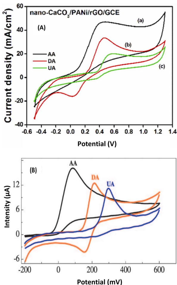
Fig. 7 (A) CVs of 3 mM AA (a), 1 mM DA (b) and 1 mM UA (c) at nano-CaCO 3 /PANI/rGO/GCE (B) in PB (0.1 M, pH 6). Scan rate: 100 mV s -1 . This figure has been reproduced from ref. 23 with permission from Elsevier Ltd., copyright 2022. (B) CVs at chitosan-graphene/GCE in 0.05 M PBS (pH 7.0) containing 2 mM AA (black line) or 1 mM DA (red line) or 0.5 mM UA (blue line). Scan rate: 50 mV s -1 . This figure has been reproduced from ref. 47 with permission from Wiley-VCH Verlag GmbH & Co. KGaA, copyright 2010.
