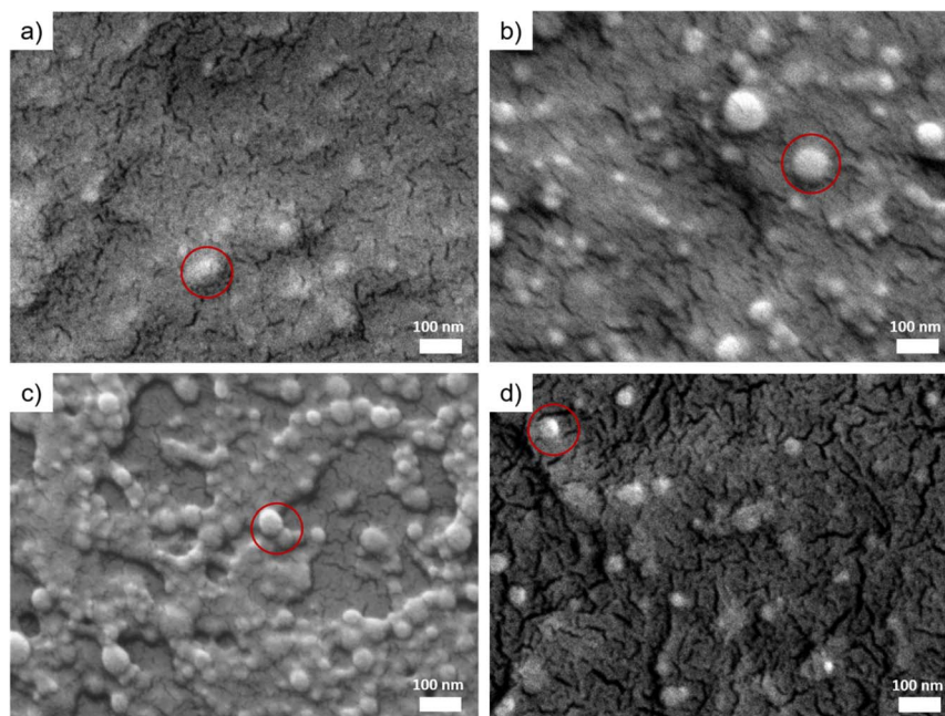
Fig. 3 SEM images of CLP-based samples. (a) CLP 20P. (b) CLP/H 2 O 20P. (c) CLP on CNF 20P. (d) CLP/CNF 20P. The red rings indicate colloidal lignin nanoparticles.
