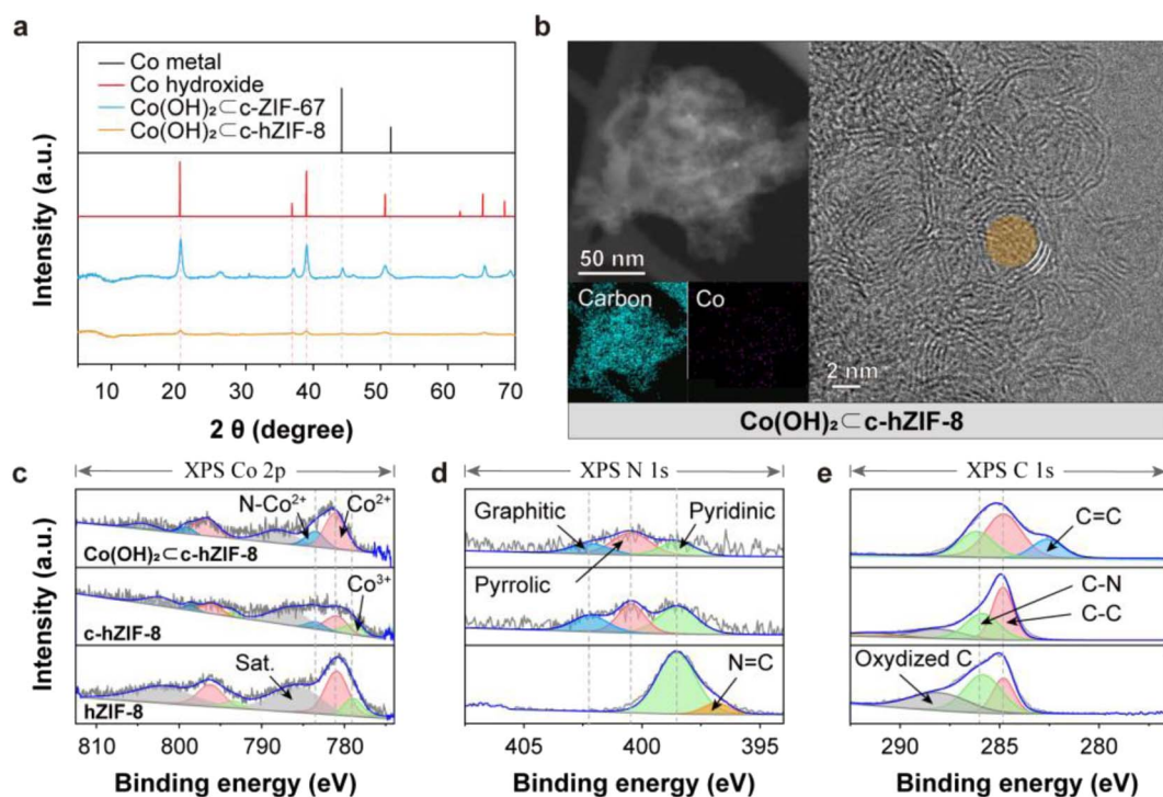
Fig. 3 Chemical characteristics of hZIF-8, c-hZIF-8, and Co(OH) 2 ⊂c-hZIF-8. (a) Comparison of XRD patterns of Co metal and Co(OH) 2 for Co(OH) 2 ⊂c-ZIF-67 and Co(OH) 2 ⊂c-hZIF-8. (b) STEM and EDS images of Co(OH) 2 ⊂c-hZIF-8. (c–e) Co 2p, N 1s, and C 1s XPS core level spectra of the as-synthesized hZIF-8, c-hZIF-8, and Co(OH) 2 ⊂c-hZIF-8.
