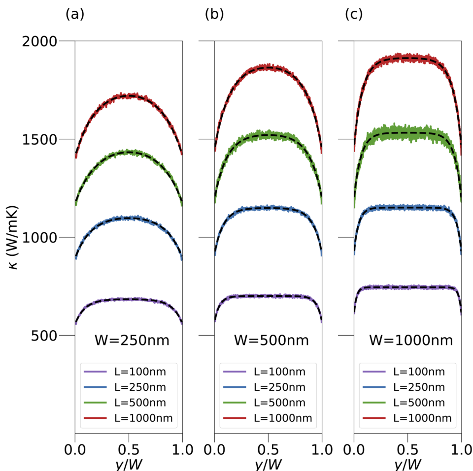
Fig. 2 Length-averaged position-dependent thermal conductivity \kappa (in units of W\text{ mK}^{-1} ) along width: (a) W = 250 nm, (b) 500 nm and (c) 1000 nm, respectively. The black dashed lines represent the fitting function in eqn (3).
