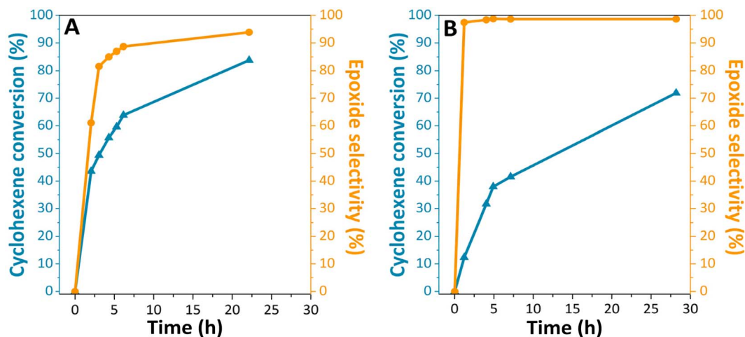
Fig. 4 Conversion of cyclohexene (blue) and epoxide selectivity (yellow) results from catalytic tests of the \text{TiO}_2@SiC/SiO_2-p catalyst with (A) tert -butyl hydroperoxide and (B) cumene hydroperoxide as the oxidant.
