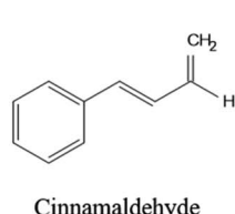
Cinnamaldehyde
