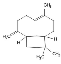
Caryophyllene
