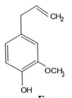
Eugenol
