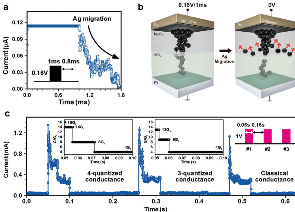
Fig. 4 The Ag migration after a pulse of 0.16\text{ V}/1\text{ ms} . (a) The exponential decay was observed because the unstable Ag filament diffused at around 0.8\text{ ms} . (b) A schematic representation of before and after the Ag migration. The metal filament was formatted by the 0.16\text{ V}/1\text{ ms} pulse but metal ions diffused after the pulse. (c) The quantum conductance for the stimulation with the pulse, 1\text{ V}/0.05\text{ s} . The conductance was calculated by the equation, G_0 = 2e^2/h . During applying the first pulse, 4-quantized conductance was observed with 16, 14, 8, and 4G_0 . Secondly, the conductance was identified by 3-quantized steps with 13, 9, and 4G_0 and finally decreases classically.
