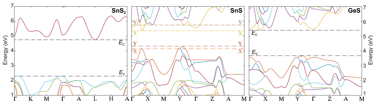
Fig. 5 Energy-aligned band structures of SnS 2 , SnS, and GeS, showing the different band offsets. The E(k) dispersion relations of the valence- and conduction bands of the three layered semiconductors were calculated using density functional theory with identical methodology (PBE-D2 with G_0W_0 quasiparticle corrections, see Methods) and their energy axes were aligned via the electrostatic potential from interface models of vertical SnS–SnS 2 and SnS–GeS van der Waals stacks (see Fig. S8, ESI ^\dagger ) to reflect the actual band offsets between the different valence- and conduction band extrema. Dashed and dash-dotted lines represent the conduction band minima ( E_c ) and valence band maxima ( E_v ), respectively. For SnS, the extrema at the X- and Y-valleys are indicated with brighter and darker colors, respectively. For an illustration of the Brillouin zones of the three crystals and designation of the high-symmetry points, see Fig. S7 (ESI ^\dagger ).
