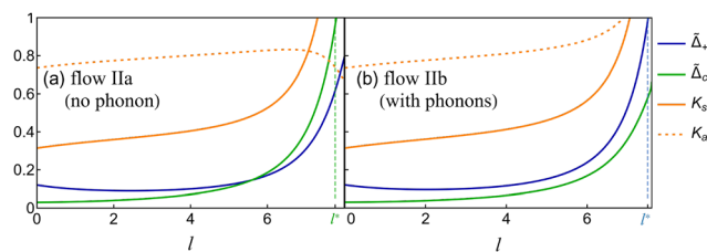
Fig. 3 Comparison of RG flows without and with phonon influence for \tilde{A}_+(0) = 4\tilde{A}_c(0) = 0.12 , U_{ee}/(\pi\hbar v_F) = 2.5 and V_{ee}/U_{ee} = 0.83 . (a) RG flow corresponding to dot IIa in Fig. 2 and 4(a). (b) RG flow with v_g^2/(cv_F) = 0.53 , corresponding to dot IIb in Fig. 4(a).
