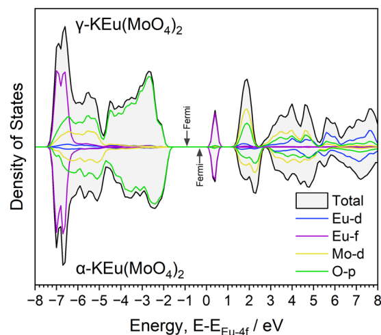
Fig. 5 Partial DOSs of the (up) \gamma\text{-KEu}(\text{MoO}_4)_2 and (down) \alpha\text{-KEu}(\text{MoO}_4)_2 .
