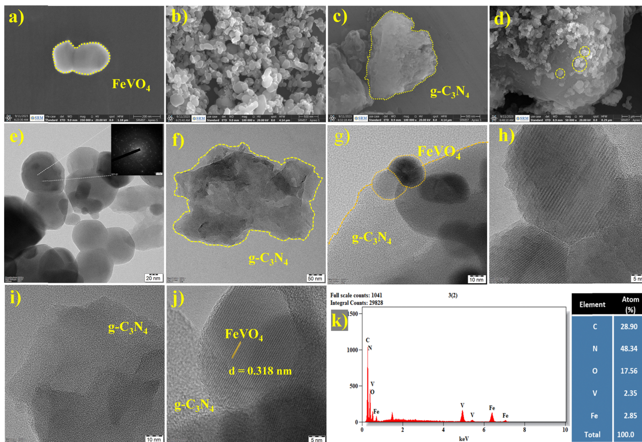
Fig. 3 SEM Micrographs of (a) and (b) FVO (FeVO 4 ), (c) CN (g-C 3 N 4 ), (d) FVO/CN, – TEM micrographs of (e)–(g) FVO, CN and FVO/CN, (h)–(j) lattice fringes of FVO, CN and FVO/CN, (k) EDX analysis of FVO/CN.
