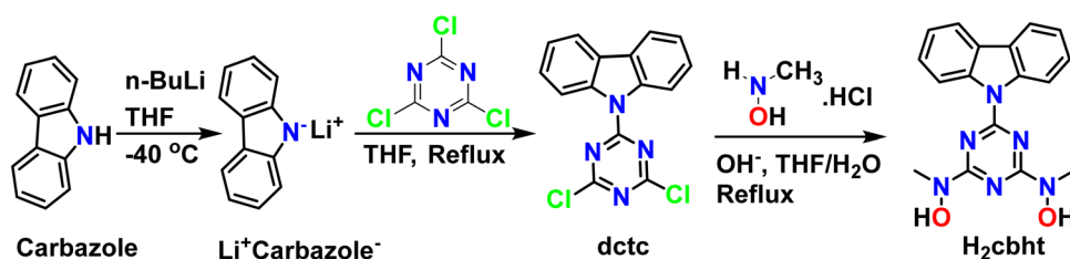
Scheme 2 Synthesis of organic molecules dctc and \text{H}_2\text{cbht} .
