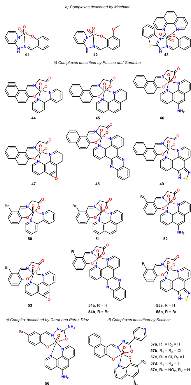
Figure 5. Vanadium pincer complexes with antiparasitic activity.
