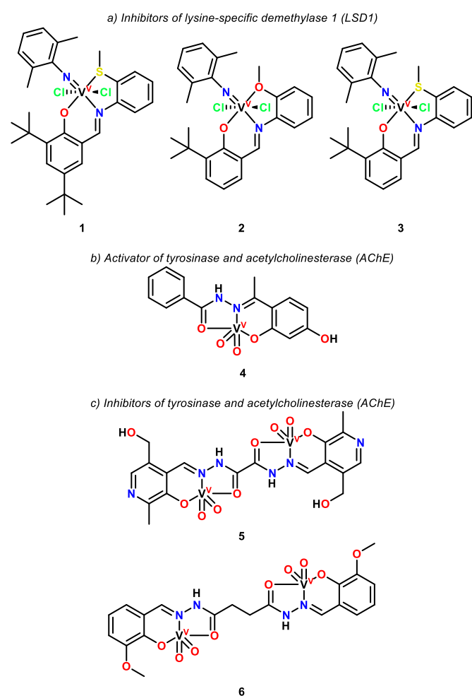
Figure 1. Vanadium compounds used as: a) LSD1 inhibitor, b) tyrosinase and acetylcholinesterase (AChE) activator, and c) enzyme inhibitors. The counterions of complexes 4–6 were omitted for clarity. Complexes 4 and 6 are triethylammonium derivatives, while complex 5 is a protonated DBU salt.
