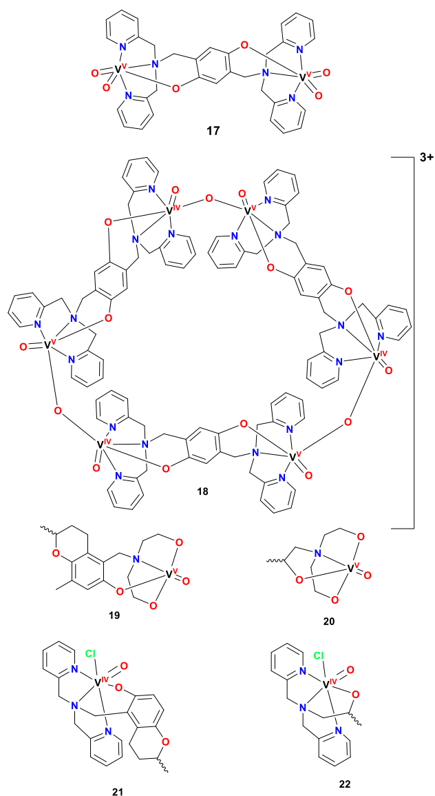
Figure 2. Vanadium pincer complexes with antioxidant activity 7-14 and oxidativ activity 15-22.
