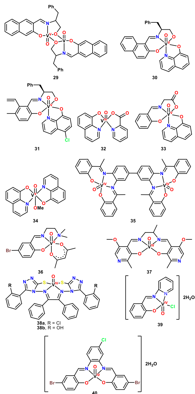
Figure 4. Vanadium pincer complexes with antibacterial and antiviral activity.
