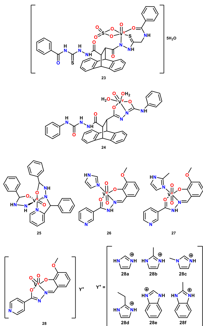
Figure 3. Vanadium pincer complexes with antidiabetic activity.
