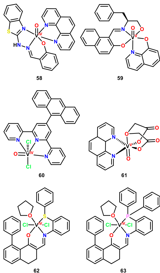
Figure 6. Example of vanadium complexes with anticancer activity.
