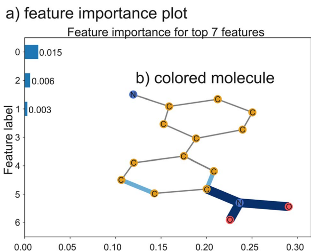
Fig. 13 Generated explanation of a SAR model using GNNExplainer. 371 A GNN was trained on the MUTAG dataset which contains the mutagenetic data of nitroaromatic compounds. The subsequent predictions were explained with GNNExplainer. The methods to do this were based off of the blog post Why should I trust my Graph Neural Network? and its associated colab. 379 (a) A feature importance plot generated by GNNExplainer for the compound. (b) Visualization of the explanation for this compound. Edges (the bonds) colored blue indicate high mask areas that the model deemed important for the prediction task. The darker the blue, the more important the bond was. For this molecule, NO 2 , a known mutagenetic substructure, 380 was highlighted as important when predicting the molecule as mutagenetic.
