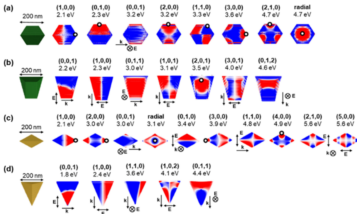
Fig. 2 Calculated near-field charge distribution of resonant modes in tent and kite shapes of Mg NPs. Plasmon modes of (a) tent, (b) filled tent, (c) (1121) kite and (d) filled (1121) kite where blue and red colours (arbitrary intensity) correspond to opposite charges on the NP's surface. Electron beam excitation is denoted by a black circle at the beam position, with propagation perpendicular to the page, while for photon excitation, the incident field direction ( k , single arrow) and polarisation ( E , double arrow) are shown. Incident field directions and polarisations perpendicular to the page are denoted with \otimes and a k or E annotation.
