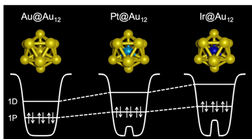
Fig. 1 Schematic illustration of the two-step jellium potential and superatomic orbitals of M@(\text{Au}^+)_{12} ( M = \text{Au}^+, \text{Pt}^0, \text{Ir}^- ). Reproduced from ref. 95 with permission from the American Chemical Society, Copyright 2020.
