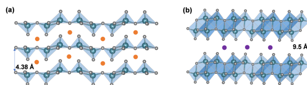
Fig. 4 Pre-intercalated \alpha - V_2O_5 into (a) “hinged” structure and (b) bilayered structures with expanded interlayer distance. Reproduced with adaption from ref. 58 with permission from Elsevier. Copyright 2019.
