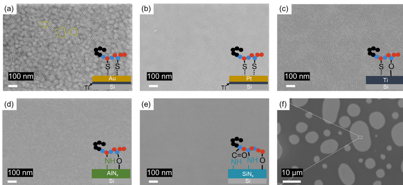
Fig. 4 (a–e) Top-down SEM images of a 26 nm thick film of S-b-G(TFET-r-2MP) annealed on different surfaces. (a) Au. (b) Pt. (c) Ti. (d) \text{AlN}_x . (e) \text{SiN}_x . In (a), the yellow dashed circles indicate the grain-like structure. A thin layer of Ti was also used as an adhesion layer when creating the Au and Pt substrates. (a) and (b) show a thin film of Ti between the metal and the Si, which was used as an adhesion promoter. The image in (e) is featureless because the assembled film lacks perpendicular domains. (f) Large-area SEM image of a self-assembled thin film of 26 nm thick S-b-G(TFET-r-2MP) on \text{SiN}_x that exhibits island and hole topographic features, indicative of a parallel domain orientation at the free surface.
