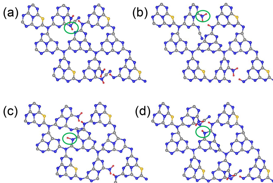
Fig. 1 Optimized structures of dual defect ON-GCN tautomers. The structures are labeled based on the position of the circled hydrogen atoms as (a) NH–CN (most stable structure), (b) NH 3 , (c) N_Hβ and (d) N_Hα (least stable structure), Table 1. C: grey, N: blue, O: golden and H: red.
