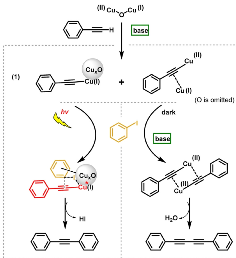
Fig. 10 Sonogashira and Glaser coupling reaction pathways over the \text{Cu}_x\text{O/CNT} catalyst under light irradiation and dark conditions respectively. "Reproduced from ref. 89 with permission from Elsevier, copyright 2022".
