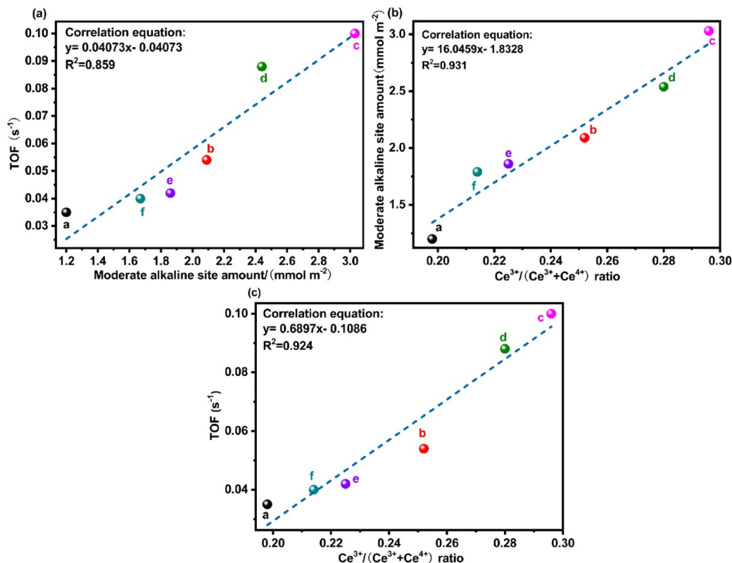
Fig. 8 (a) Correlation between the TOF values at 250 °C and the amount of surface moderate alkaline sites, (b) the correlation between the surface moderate alkaline sites and Ce^{3+}/(Ce^{3+} + Ce^{4+}) ratio, and (c) the correlation between the TOF values at 250 °C and Ce^{3+}/(Ce^{3+} + Ce^{4+}) ratios. (a) Ni/CeO 2 ; b. Ni/Ca 0.05 Ce 0.95 O y ; c. Ni/Ca 0.1 Ce 0.9 O y ; d. Ni/Ca 0.125 Ce 0.875 O y ; e. Ni/Ca 0.25 Ce 0.75 O y ; f. Ni/Ca 0.4 Ce 0.6 O y ). The lattice capacity threshold effect in the presence of oxygen vacancies and moderate-strength alkali centers was primarily attributed to the lattice capacity threshold effect.
