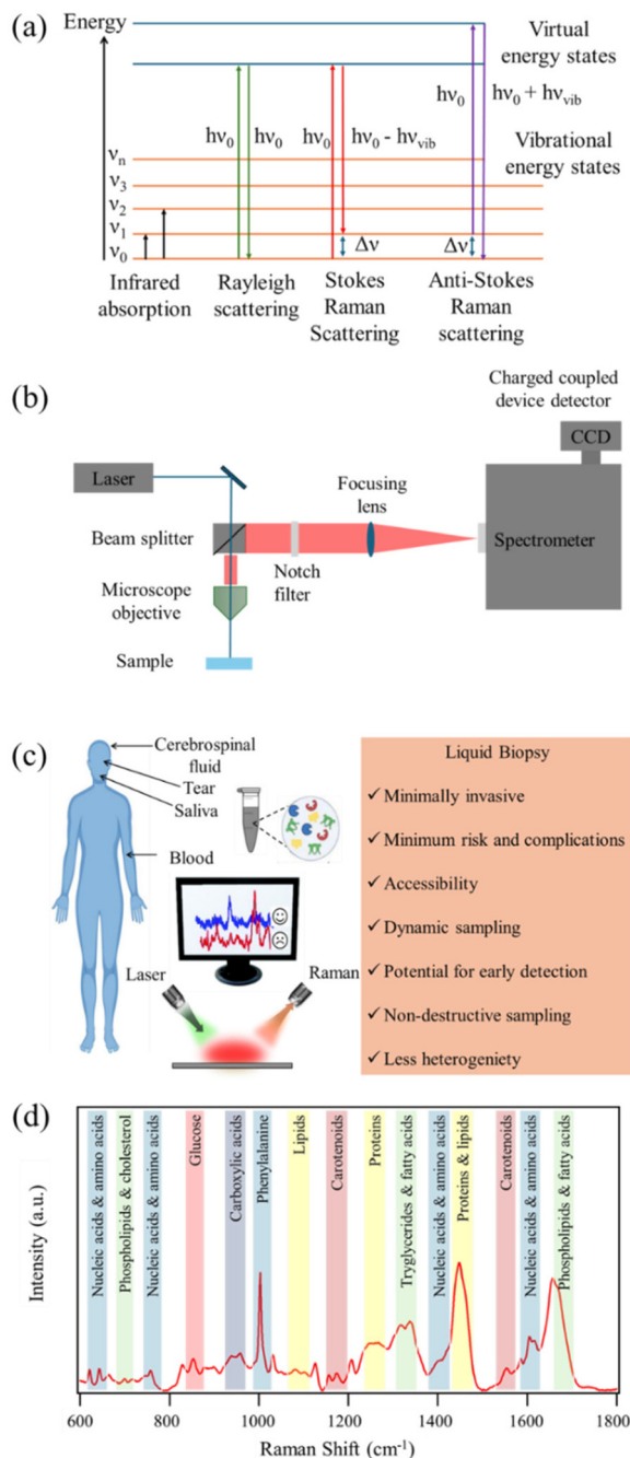
Fig. 1 (a) Schematic representation of the energy level diagram of Raman scattering process. (b) Generic setup for a Raman microscopy system. (c) Illustrative diagram depicting the use of RS in analyzing liquid biopsy for the detection and diagnosis of brain disorders. (d) Raman spectra of human serum from a healthy donor highlighting the peak assignment for various metabolic groups and biomolecules.
