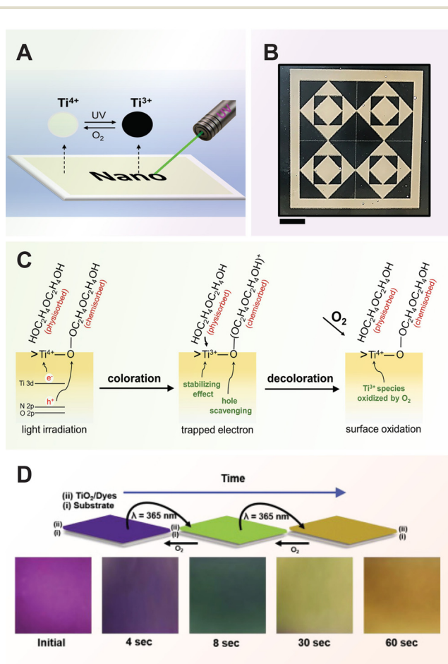
Fig. 10 Photochromic function of TiO 2 semiconductor. (A) Schematic illustration of the writing process on the rewritable paper using a laser pen and (B) light-printed pattern on rewritable film using a UV lamp. (C) Photoreversible color-switching mechanism of N-doped TiO 2 nanocrystals. Reproduced with permission from ref. 359. Copyright 2022, Wiley-VCH. (D) Color-switching process and the corresponding color change of the film under continuous UV irradiation. Reproduced with permission from ref. 356. Copyright 2019, Elsevier.
