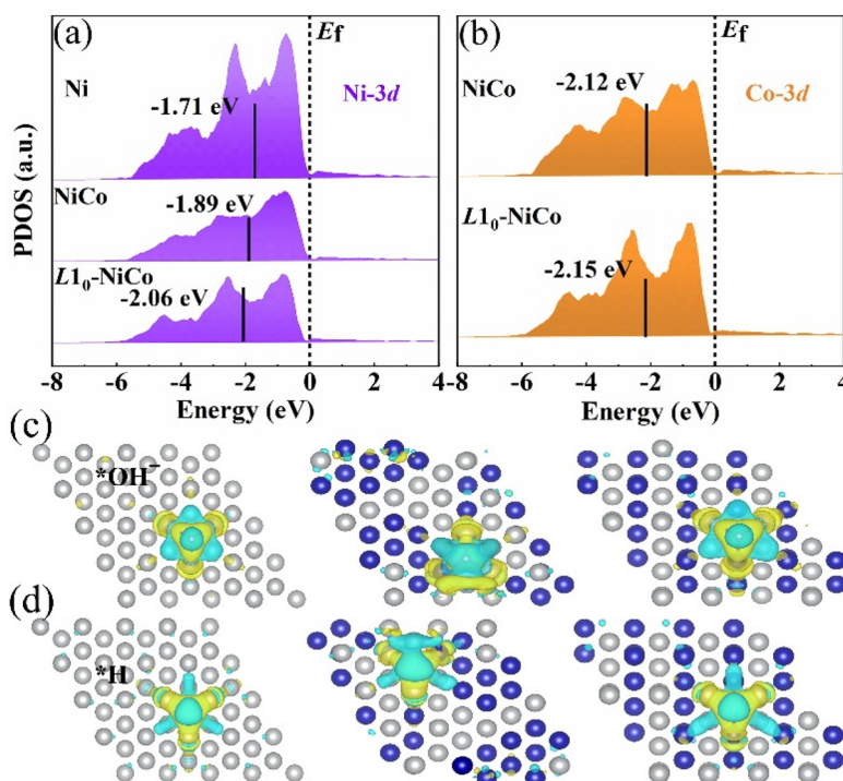
Fig. 2 (a) The density of states and d-band center of Ni and (b) Co atoms, (c) the differential charge density diagram of ^*\text{OH}^- and (d) ^*\text{H} of Ni, disordered NiCo solid solution and ordered intermetallic L_{10} -NiCo.
