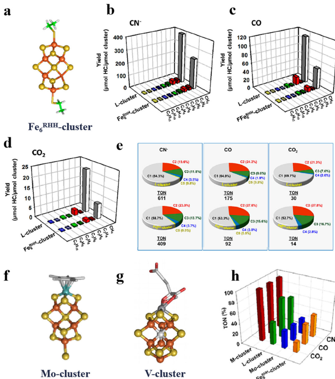
Fig. 6 Artificial Fe–S clusters based on configuration design to improve catalytic performance. (a) Structure of \text{Fe}_6^{\text{RHH}} -cluster. Types and yields of L- and \text{Fe}_6^{\text{RHH}} -clusters for the reduction of (b) \text{CN}^- , (c) CO and (d) \text{CO}_2 to hydrocarbons. (e) L- and \text{Fe}_6^{\text{RHH}} -clusters percentage of products forming hydrocarbons. (f) Structure of Mo-cluster. (g) Structure of V-cluster. (h) TON of M-, L-, Mo- and \text{Fe}_6^{\text{RHH}} -clusters for the reduction of \text{CN}^- , CO and \text{CO}_2 . Reproduced with permission from ref. 36. Copyright 2017, American Chemical Society.
