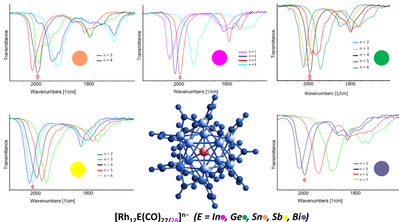
Fig. 8 Multivalence behaviour of the [Rh 12 E(CO) 27/28 ] n- family of clusters ( n = 3 when E = In, Sb, Bi; n = 4 when E = Ge, Sn) as obtained by spectro-electrochemical experiments. 27
