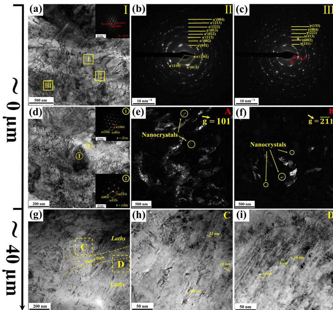
Fig. 4 Transmission electron microscopy (TEM) characterization of the USPped sample with the peening duration of 8 min. (a) Bright-field (BF) image of the sample at its topmost surface, the right-upped corner inset shows the selected area electron diffraction (SAED) patterns of area I in (a); SAED patterns of (b) area II and (c) area III as marked in (a); (d) magnified BF observation of the USPped sample at its topmost surface, the right-upped and right-lower insets show the SAED patterns of the \alpha phase and \gamma phase marked as areas ① and ②, respectively; (e) and (f) dark-field images of the \alpha phase and \gamma phase with the \vec{g} of 10\bar{1} and 2\bar{1}1 , respectively; (g) BF image of the USPped sample at the location of 40\mu\text{m} depth from its topmost surface; and (h) and (i) magnified BF images at that area showing that the lath-shaped phases have refined into several nanometers in thickness.
