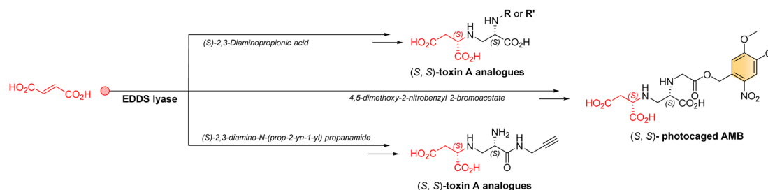
Fig. 1 Synthesis of complex aminopolycarboxylic acids. (I) Previous chemical, chemoenzymatic and biocatalytic synthesis strategies towards the aminopolycarboxylic acid AMA and (II) our chemoenzymatic synthesis strategies towards related aminopolycarboxylic acids ( i.e. , toxin A derivatives).
