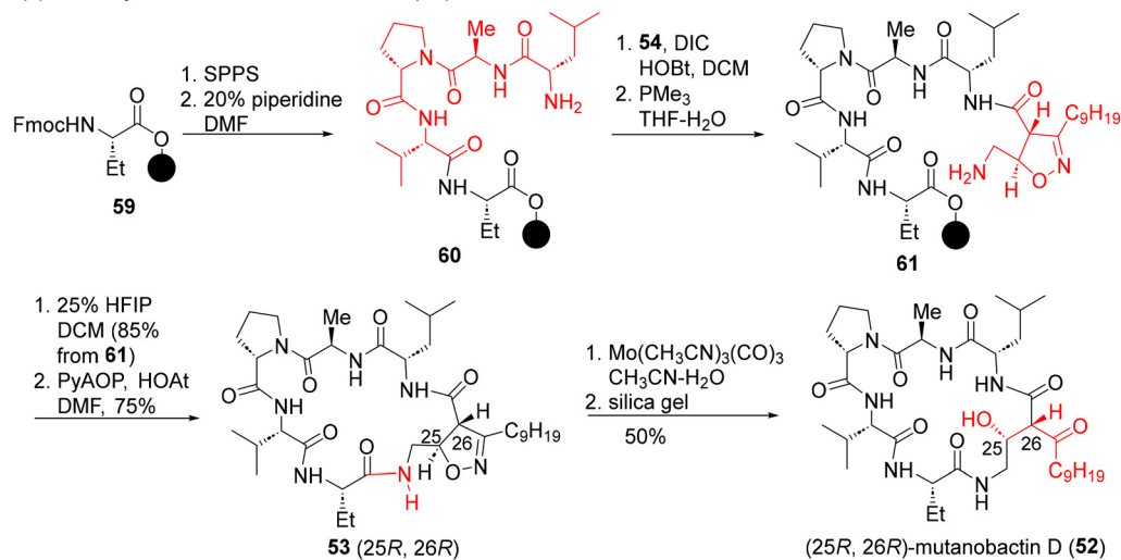
(c) Total synthesis of mutanobactin D ( 52 )
