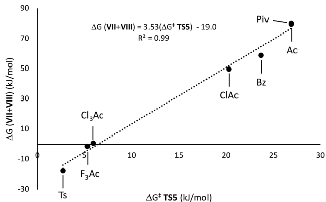
Fig. 2 Free energy of activation ( \Delta G^\ddagger , \text{kJ mol}^{-1} ) for TS5 vs. reaction energy for heterolytic dissociation ( \Delta G(\text{VII} + \text{VIII}) , \text{kJ mol}^{-1} ) for carboxylate and sulfonate groups ((U)M06-2X/def2-TZVP//SMD(acetonitrile) level of theory).
