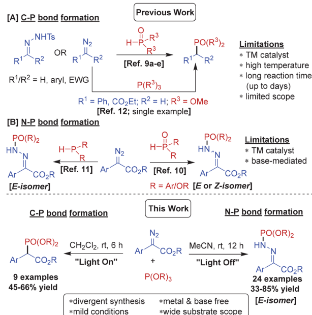
Scheme 1 Carbon vs. nitrogen phosphorylation of diazo compounds.
