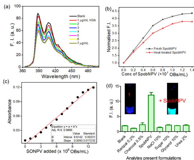
Fig. 5 (a) Fluorescence titration of 1 ( 10 \mu M, \lambda_{\text{ex}} = 370 nm) in the presence of HSA ( 0 – 7 \mu g \text{mL}^{-1} ) in water. (b) Change in the emission spectra of 1 ( 10 \mu M, \lambda_{\text{ex}} = 454 nm) in the presence of fresh and heat-treated SpobNPV ( 0 – 1.3 \times 10^7 OBs \text{mL}^{-1} ) in water. (c) Change in the absorbance of compound 1 ( 10 \mu M) at 454 nm upon adding SpobNPV ( 0 – 1.3 \times 10^7 OBs \text{mL}^{-1} ) in water. (d) Change in the emission intensity of 1 ( 10 \mu M, \lambda_{\text{ex}} = 370 nm) at 510 nm in the presence of different analytes present in commercial formulations.
