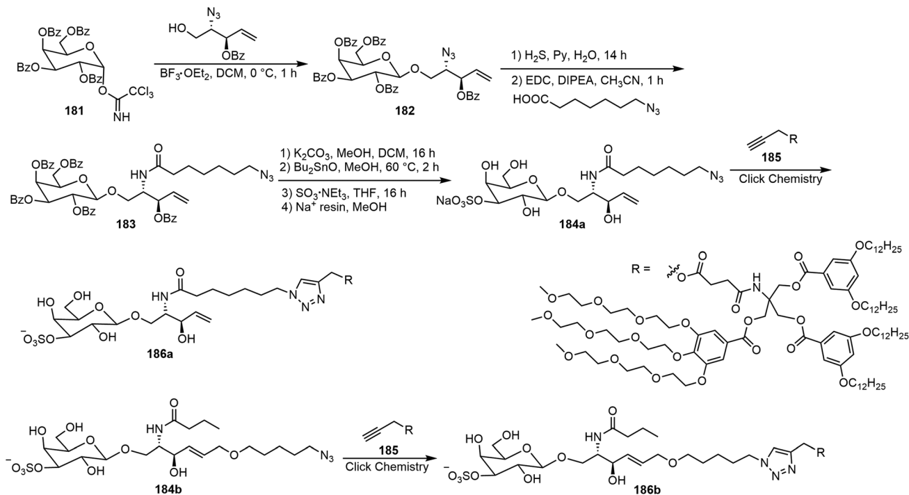
Scheme 28 Synthesis of sulfate-substituted galactose-containing glycodendrimeres 186 .
