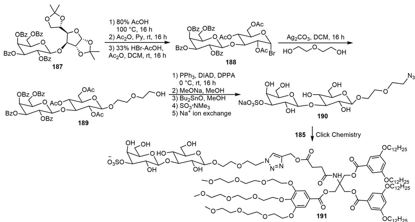
Scheme 29 Synthesis of sulfate-substituted lactose-containing glycodendrimer 191 .
