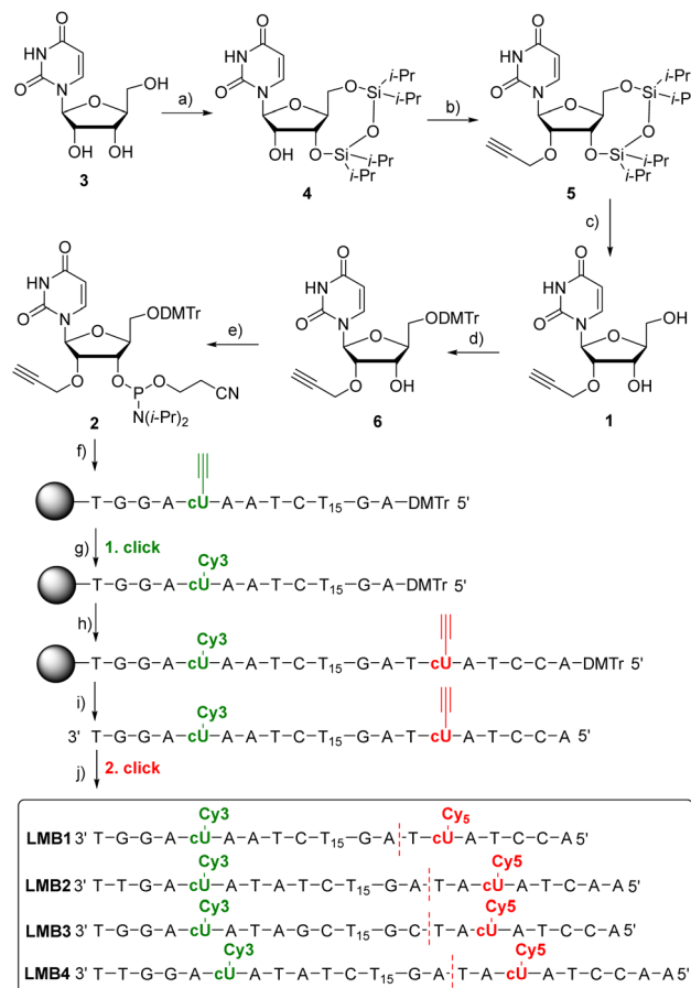
Fig. 2 Synthesis of 1 and 2 and the sequences of LMB1 – LMB4 . (a) TIPDSiCl 2 , pyridine, 2 h, 0 ^{\circ}\text{C} then r.t., o.n., 80%; (b) 1. NaH, THF, -10\text{ }^{\circ}\text{C} , 15 min; 2. propargyl bromide, r.t., o.n., 54%; (c) 1 M TBAF/THF, THF, r.t., 5 min, quant.; (d) DMTr-Cl, pyridine, r.t., o.n., 80%; (e) 2-cyanoethyl- N,N -diisopropylchlorophosphoramidite, (iPr) 2 NEt, CH 2 Cl 2 , r.t., 3 h, 85%; (f) automated DNA synthesis on the solid phase (CPG), (g) Cy3-azide, (CH 3 CN) 4 Cu(PF 6 ), sodium ascorbate, DMSO : tBuOH : MeCN, 60 ^{\circ}\text{C} , 2 h; (h) automated DNA synthesis on the solid phase (CPG); (i) NH 4 OH, H 2 O, 55 ^{\circ}\text{C} , o.n.; (j) TBTA, (CH 3 CN) 4 Cu(PF 6 ), sodium ascorbate, DMSO : tBuOH : MeCN, 60 ^{\circ}\text{C} , 2 h. For details see the ESI (Fig. S1–S20).† The D-configured molecular beacons DMB1 and DMB4 have sequences identical to those of LMB1 and LMB4 , respectively, but are made completely of D-configured nucleotides.
