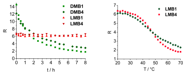
Fig. 4 Time-dependent fluorescence intensity ratio R = I_{A668}/I_{D565} of the molecular beacons LMB1 , LMB4 , DMB1 and DMB4 in the cell lysate (left, 2.5 \mu M, \lambda_{exc} = 518 nm) and the temperature-dependent fluorescence intensity ratio R of the molecular beacons LMB1 and LMB4 in the cell lysate (right, 2.5 \mu M, \lambda_{exc} = 518 nm).
