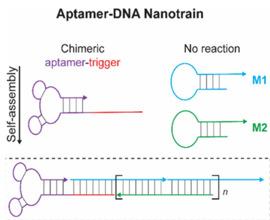
Fig. 4 Schematic representation of DNA nanostructure assembly. DNA nanotraining containing aptamers assembled by complementarity of the sequence. 138
