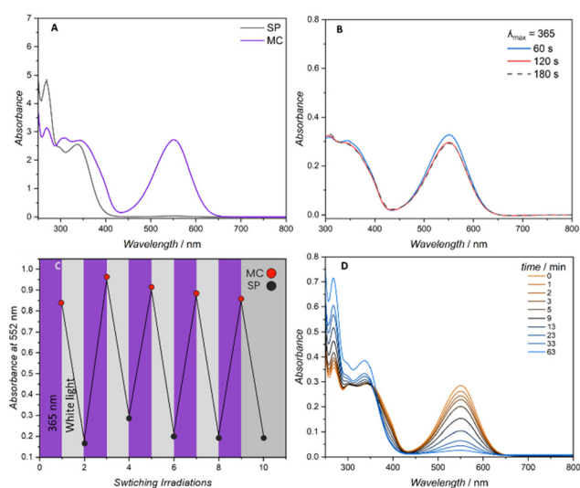
Fig. 2 UV-Vis spectroscopy of SP-36-PEGMEMA dissolved in a dioxane/methanol mixture. (A) UV-Vis of SP-36-PEGMEMA spectrum after irradiation for 1 min with a 365 nm centred LED affording the open merocyanine (MC) form of the polymeric spiropyran (SP) pendant groups, indicated by an increase in the absorption band centred at 552 nm. (B) Effect of increasing irradiation time on the generation of SP-36-PEGMEMA bound spiropyran into merocyanine units. (C) Periodic irradiation of SP-36-PEGMEMA with 365 nm and subsequent white light irradiation. The absorption band at 552 nm was used to monitor the formation of the merocyanine and spiropyran isomers. (D) Thermal relaxation in dioxane : methanol 1 : 6 of the merocyanine isomers generated by 365 nm irradiation within SP-36-PEGMEMA , monitored over 1 h by UV-Vis spectroscopy.
