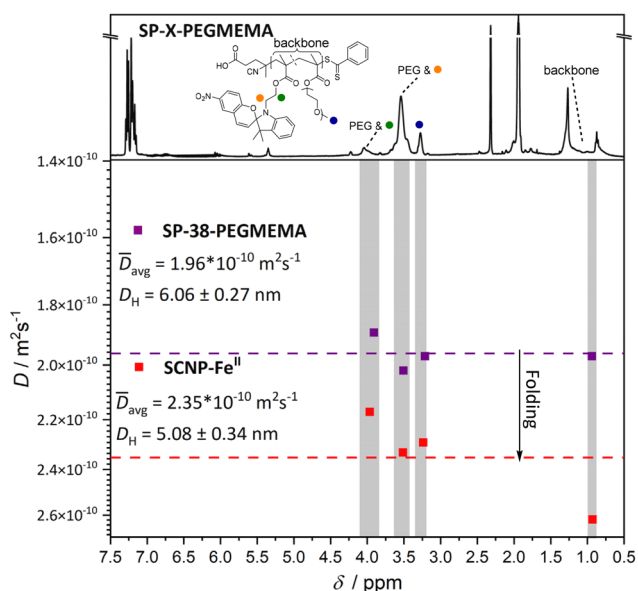
Fig. 3 DOSY spectra recorded in deuterated acetonitrile yield diffusion coefficients for both the linear polymer (SP-38-PEGMEMA) and the Fe II -SCNP generated after irradiation and addition of Fe(BF 4 ) 2 . The protons used to determine diffusion coefficients are highlighted by coloured spheres that match the corresponding resonance on the 1 H NMR spectrum (top). Protons associated with the PMMA backbone were also used, labelled as backbone in the 1 H NMR spectrum. The mean value of the diffusion coefficients calculated for the resonances – highlighted in grey – associated with both SP-38-PEGMEMA and the Fe II -SCNP are represented by a dashed line. The mean diffusion coefficients are used to calculate approximate hydrodynamic diameters. The D H decreases after irradiation and addition of Fe(BF 4 ) 2 , indicating that intramolecular folding is occurring leading to an SCNP (for the primary DOSY data of both the Fe II -SCNP and SP-38-PEGMEMA refer to ESI section 6†).
