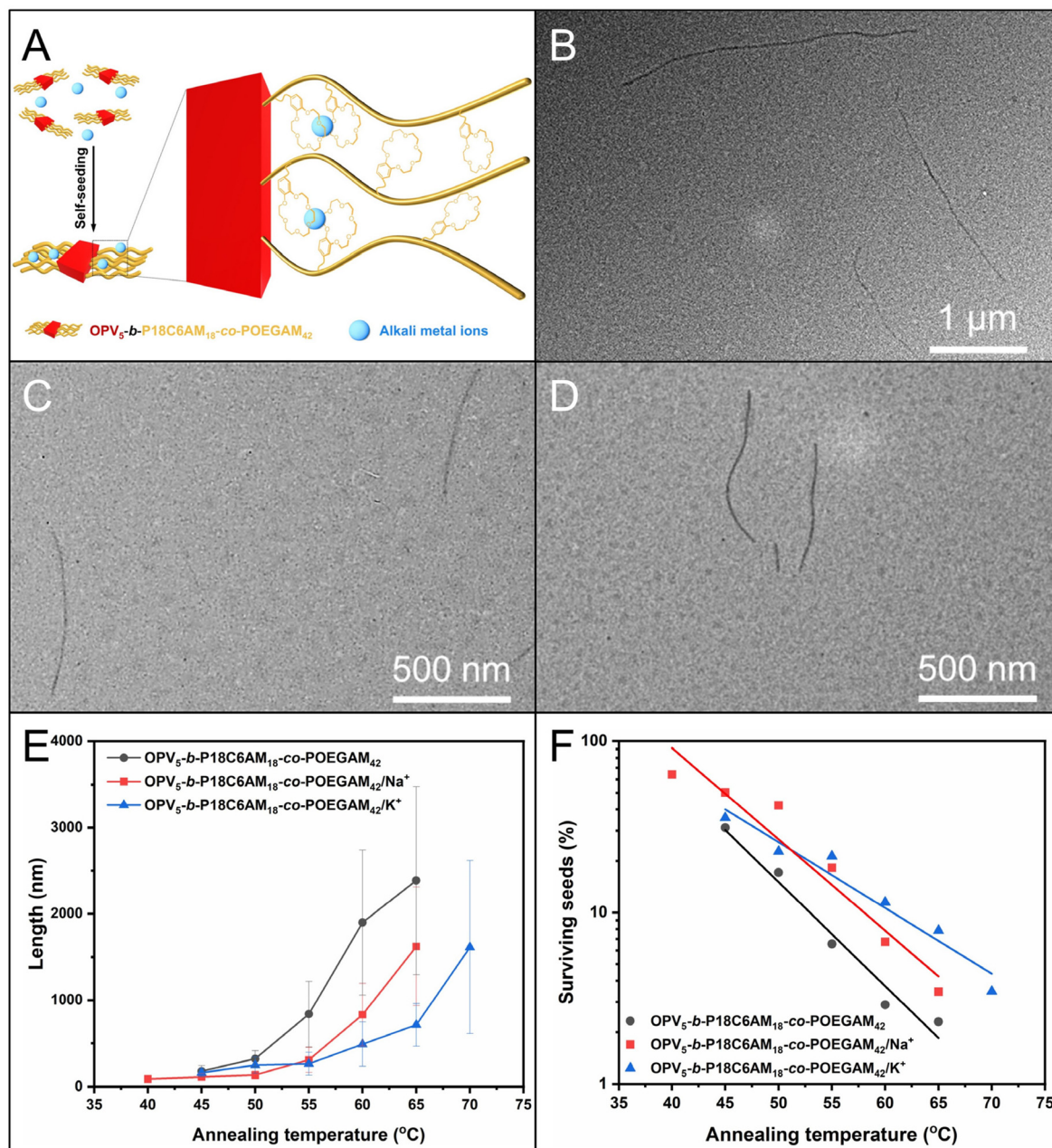
Fig. 4 (A) Schematic illustration of the self-seeding of OPV_5 - b - P18C6AM_{18} - co - POEGAM_{42} with alkali metal ions Na^+ and K^+ . Typical TEM images of the fiber-like micelles of OPV_5 - b - P18C6AM_{18} - co - POEGAM_{42} by the self-seeding approach at an annealing temperature of 60 °C (B) without and with (C) CH_3COONa and (D) CH_3COOK , respectively. (E) L_n of fiber-like micelles and (F) semilogarithmic plot of the fraction of surviving seeds of OPV_5 - b - P18C6AM_{18} - co - POEGAM_{42} versus annealing temperature ( 0.05 \text{ mg mL}^{-1} in ethanol) with and without CH_3COONa and CH_3COOK .
