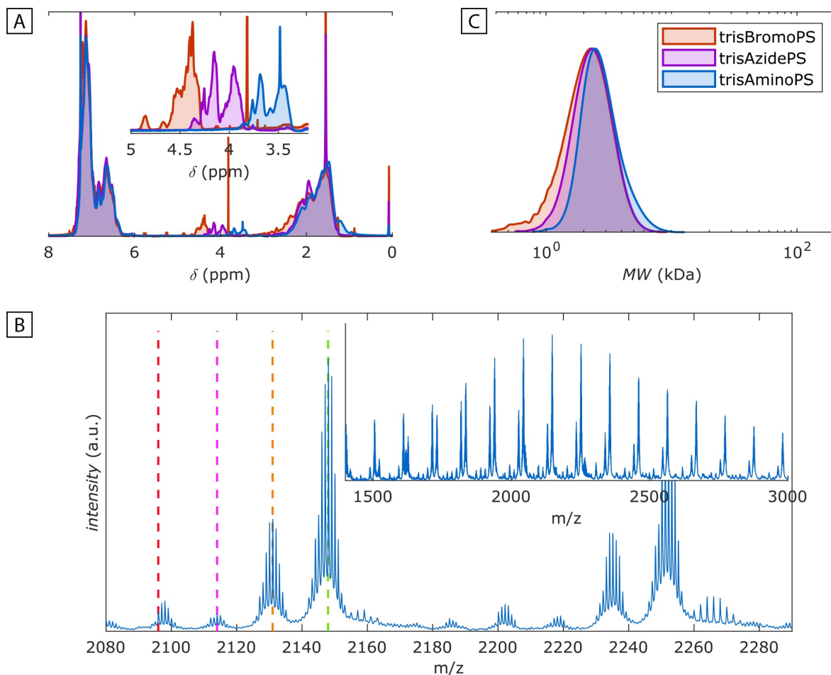
Figure 3. Characterization of a low-MW trisAminoPS ( entry 1, Table S2 ) obtained by the reduction of trisAzidePS with tributylphosphine and water. Reaction conditions: tributylphosphine (2 eq. relative to the azide functionalities of the trisAzidePS), V_{\text{THF}} = 6 \text{ mL/g} with respect to w_{\text{trisAzidePS}} , T = 60 \text{ }^\circ\text{C} , \text{time} = 0.5 \text{ h} . Subsequently, V_{\text{H}_2\text{O}} = 0.6 \text{ mL/(g)} was added, and the reaction mixture was stirred at 60 \text{ }^\circ\text{C} overnight. A) Superimposed ^1\text{H-NMR} spectra of trisBromoPS ( orange ), trisAzidePS ( purple ), and trisAminoPS ( blue ). The inset highlights the chemical shift changes of the proton(s) geminal to the respective functionalities. B) MALDI-TOF MS spectrum of trisAminoPS measured using dithranol as the matrix and AgTFA as the ionizing salt. The main population appears at m/z = 2148 \pm n \cdot 104 \text{ u} ( green dashed line ), with progressively less intense populations observed at m/z = 2131 ( orange ), 2114 ( magenta ), and 2096 ( red ) \pm n \cdot 104 \text{ u} . Assignments are discussed in the text. C) MWDs of the products.
