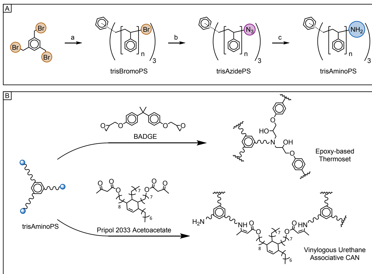
Figure 1. Overview of the reactions explored. A) Synthetic pathway yielding trifunctional primary amine-terminated polystyrene: a) ARGET ATRP of styrene initiated by 1,3,5-tris(bromomethyl)benzene, b) nucleophilic substitution with sodium azide, c) Staudinger reduction with tributylphosphine and water. B) Crosslinking process using bisphenol A diglycidyl ether
