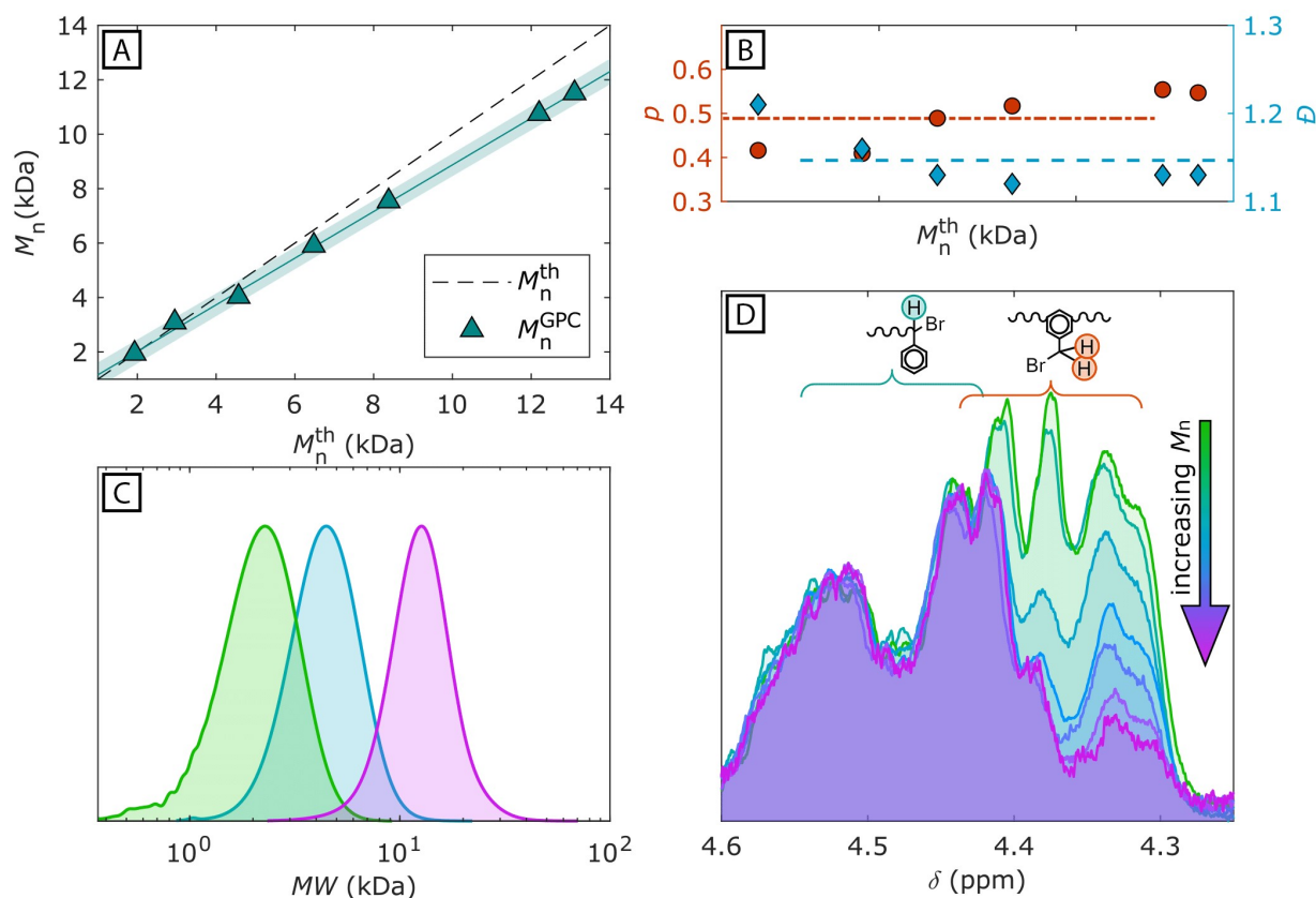
Figure 2. Characterizations of trisBromoPSs obtained via the ARGET ATRP of styrene initiated by 1,3,5-tris(bromomethyl)benzene. Reaction conditions: [\text{styrene}]_0 : [\text{CuBr}_2]/(4,4'\text{-dinonyl-2,2'-}
