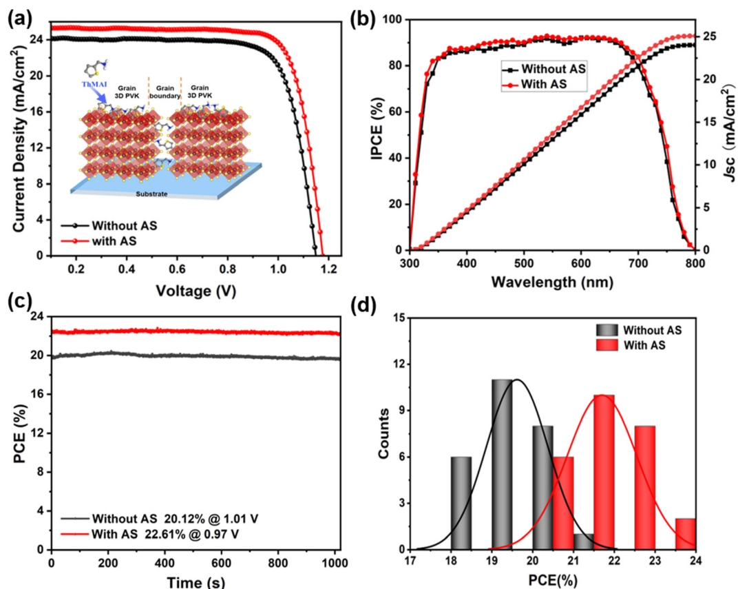
Fig. 2 (a) J - V curves (reverse scan) of champion devices fabricated without and with AS methods; (b) IPCE curves of champion devices fabricated without and with AS methods; (c) SPOs of different PSCs was operated at the maximum power point under simulated AM 1.5G sunlight of 100 \text{mW cm}^{-2} ; (d) reproducibility of 26 devices fabricated using different methods.
