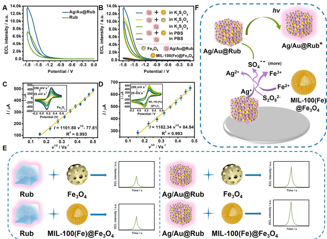
Fig. 3 (A) ECL–potential curves of Rub and Ag/Au@Rub PNCCS. (B) ECL–potential curves of Ag/Au@Rub PNCCS with \text{Fe}_3\text{O}_4 or \text{MIL-100(Fe)@Fe}_3\text{O}_4 catalyst and without catalyst in PBS containing \text{K}_2\text{S}_2\text{O}_8 or PBS. CV curves and linear relationships of electrodes modified with (C) \text{Fe}_3\text{O}_4 and (D) \text{MIL-100(Fe)@Fe}_3\text{O}_4 in 5.0 \text{mmol L}^{-1} of [\text{Fe}(\text{CN})_6]^{4-/3-} at scan rates of 25–250 \text{mV s}^{-1} . Error bars = SD ( n = 3 ). (E) Effects of porous-structure lumino-phore and catalysts. (F) Feasible ECL mechanism of the constructed CRE aptasensor.
