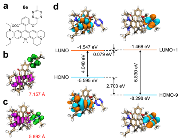
Fig. 5 (a) Molecular structure of 8e . Optimized geometries and hole–electron distributions with the corresponding d_{CT} of the ET states in (b) 8b and (c) 8c during the vertical excitation in DMSO. (d) Calculated electronic energies of different frontier orbitals in 8e during the vertical excitation in DMSO. Electron: highlighted in green; hole: highlighted in pink.
